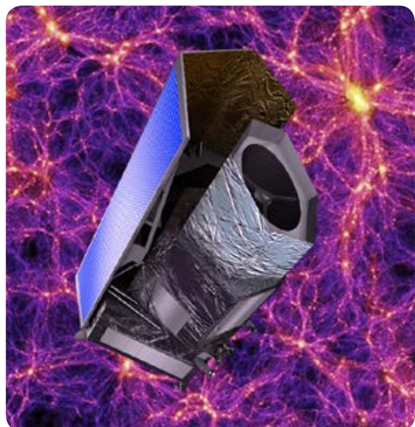
An artist's concept of the Euclid dark energy telescope in space (Credit: ESA)
