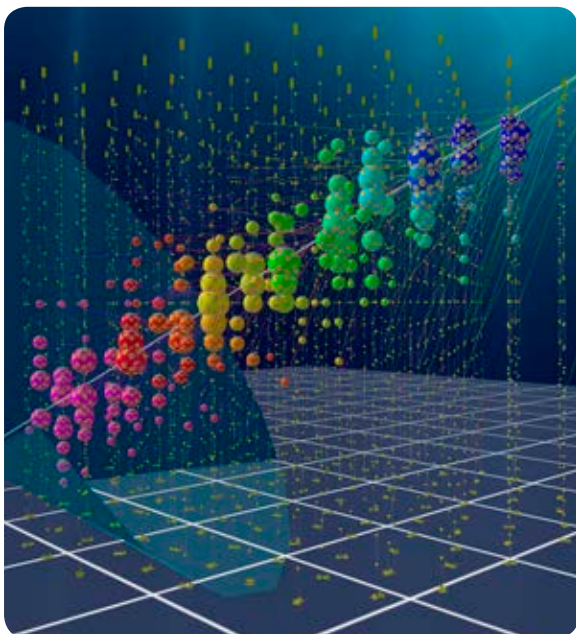
World's largest particle detector IceCube detects high-energy neutrinos from the cosmos
