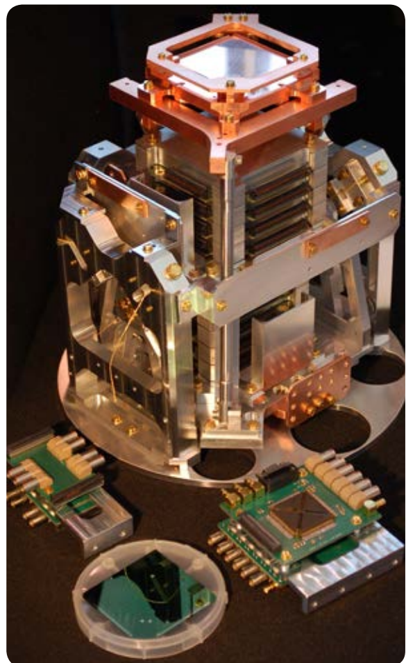
Qubic 1/4 of the focal plane
