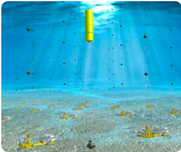
Artist's impression of Neutrino telescope KM3NeT (Credit: KM3NeT)
