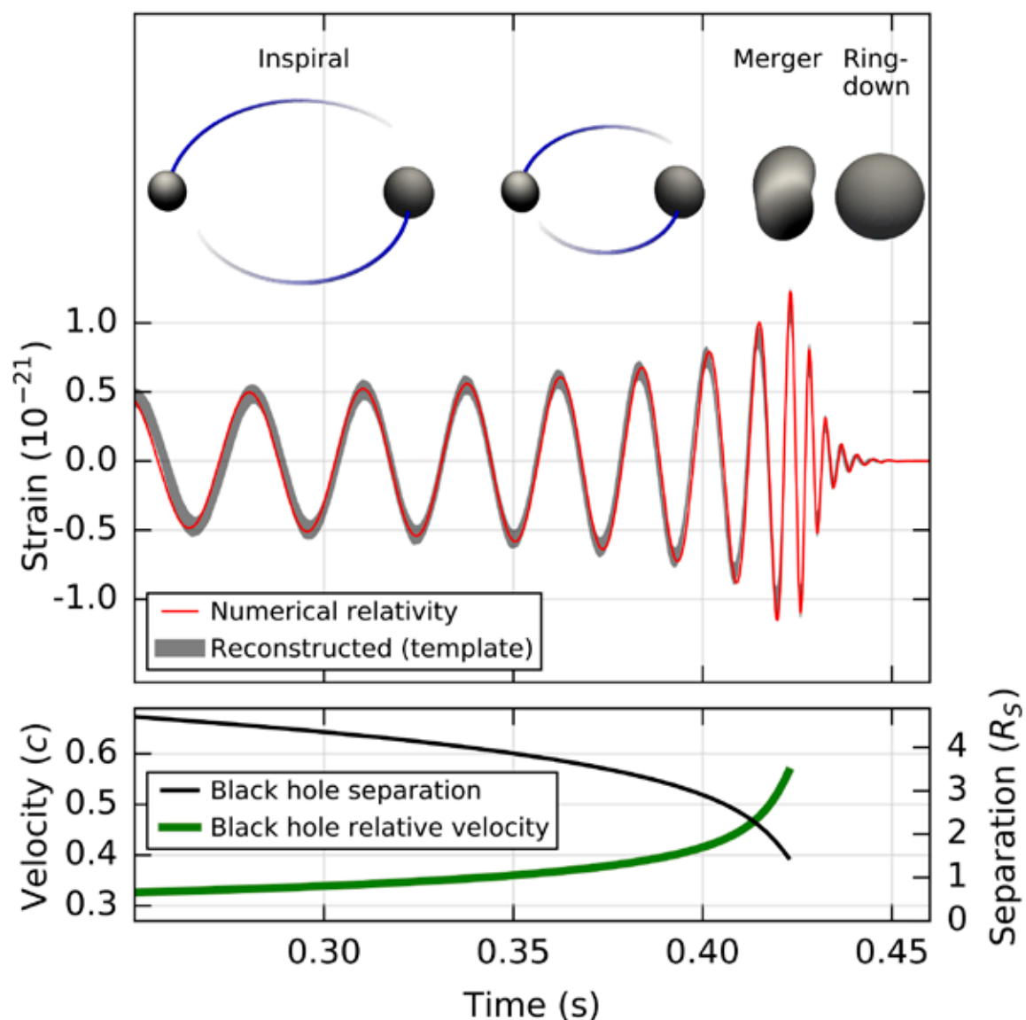
First direct observation of black holes – signal principle
