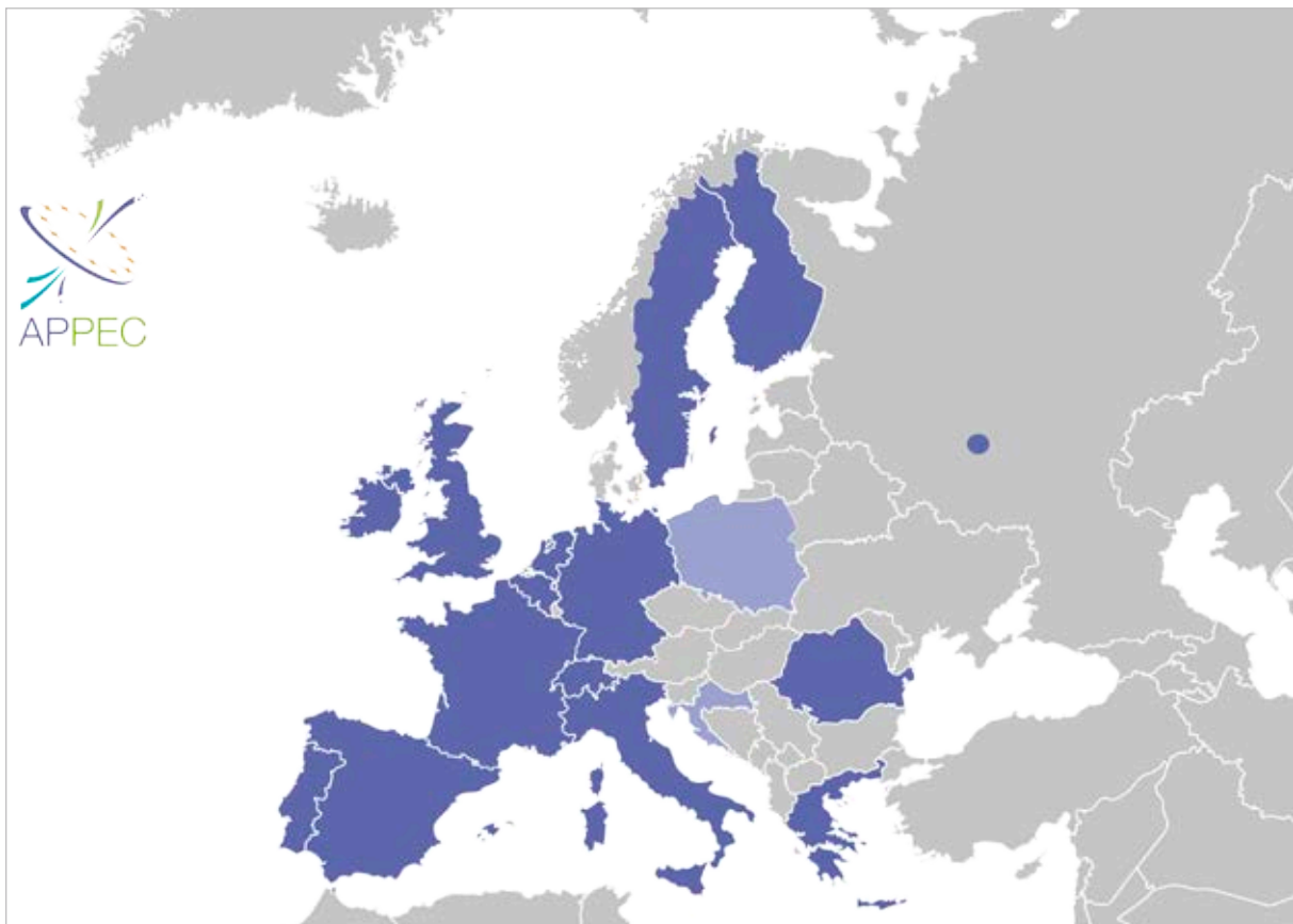
APPEC member states in 2017
