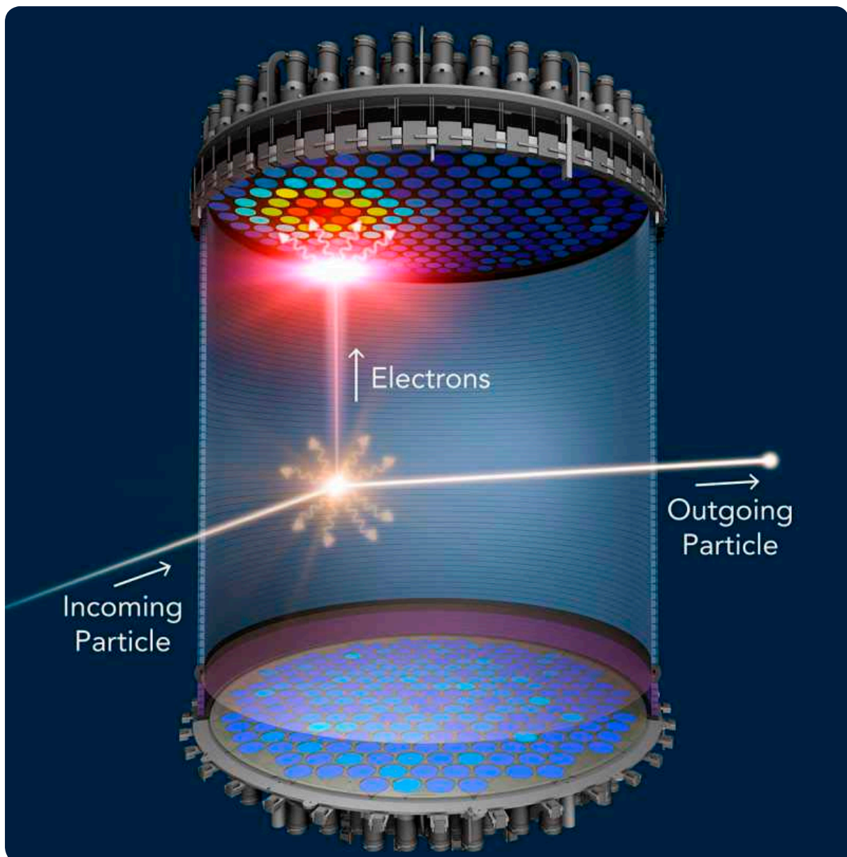
Dark Matter detection principle for Noble liquids experiments
