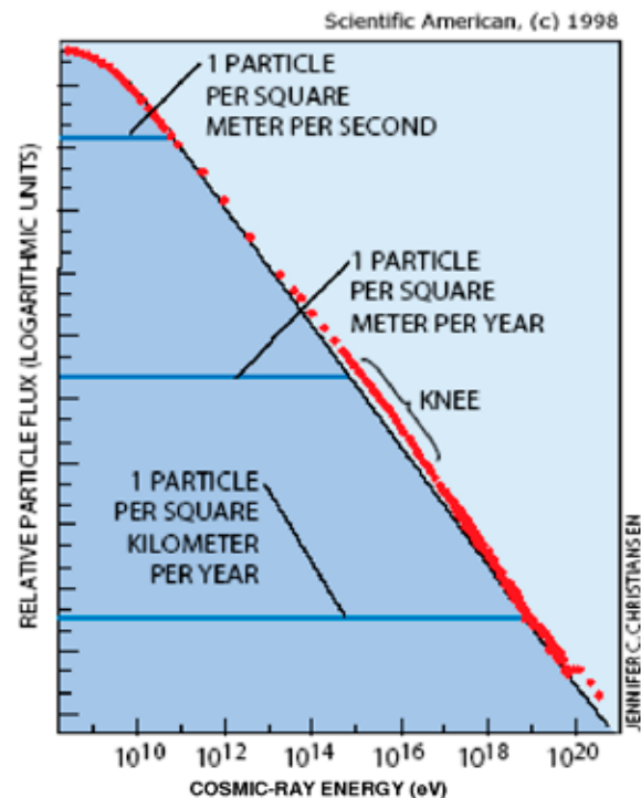
The all-particle spectrum of cosmic rays (Credit: Scientific American)
