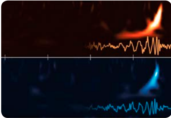
Ringing chirp: the waveform of LIGO event observed at both locations (Credit: Physics World)
