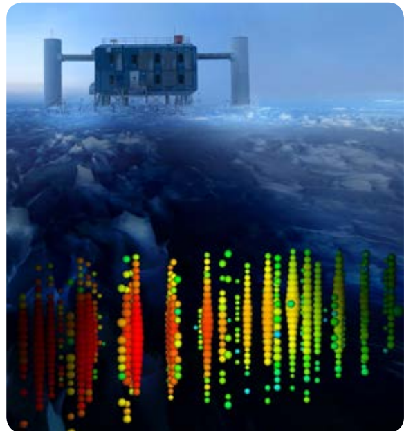
ICECUBE PeV event
