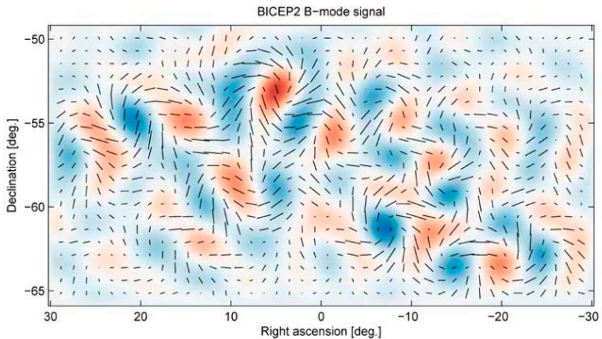
The 'curly' B-modes of polarization in the cosmic microwave background (Credit: Harvard University/BICEP2)
