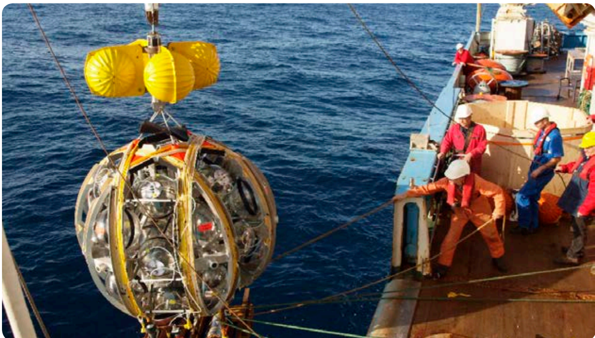
String deployment of KM3NeT (Credit: KM3NeT)
