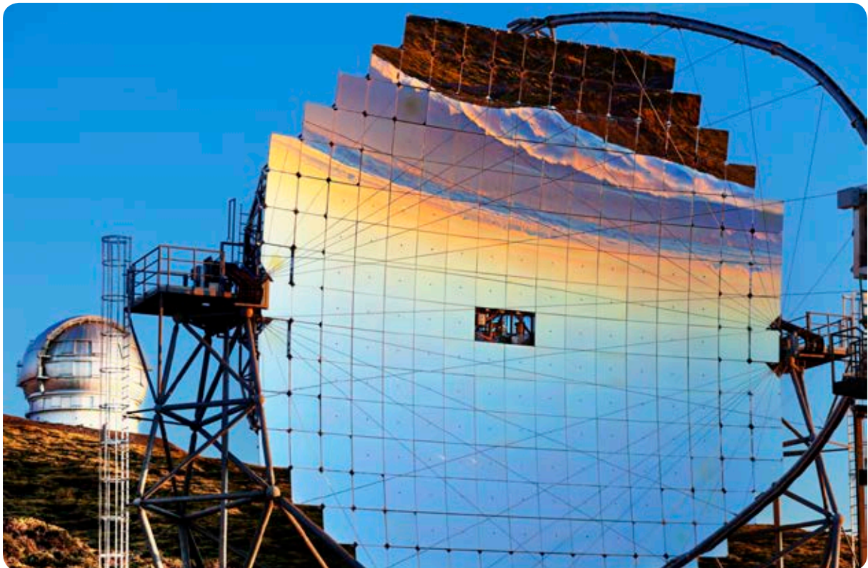
MAGIC telescope, La Palma (Credit: CTA)
