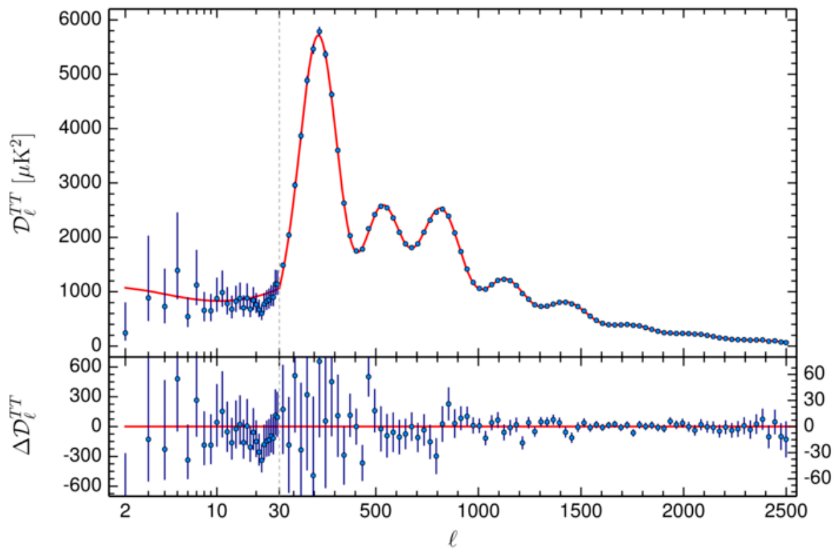
Planck power spectrum (Credit: ESA)
