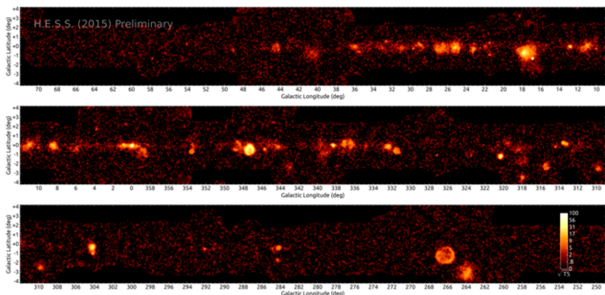
High Energy Stereoscopic System survey of the Milky Way
