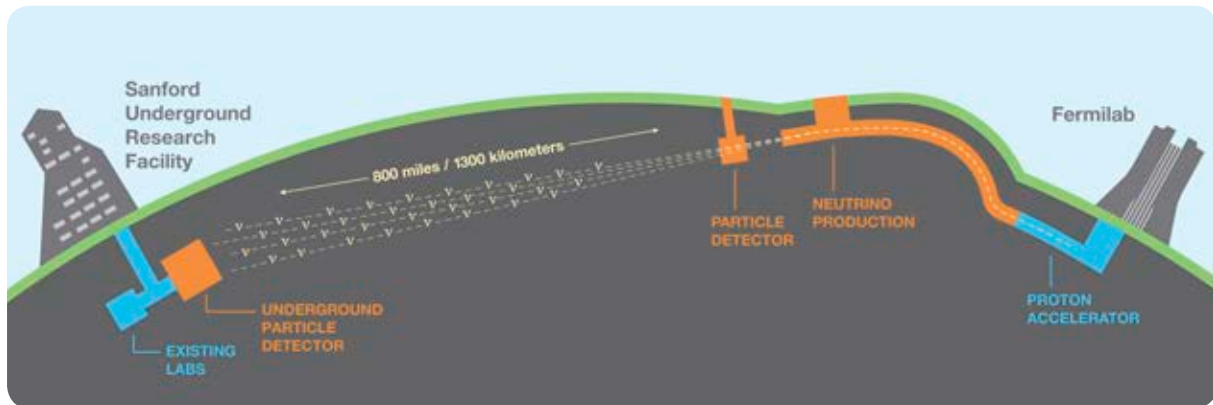
Artist's impression of the long baseline of DUNE, United States (Credit: Fermilab)
