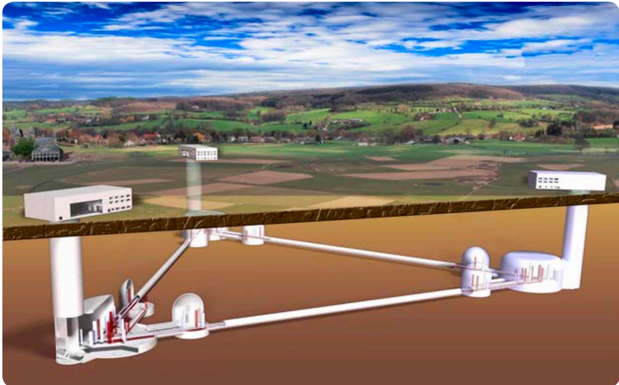
Artist's impression of the Einstein Telescope, a third-generation gravitational-wave (GW) detector (Credit: AEI)
