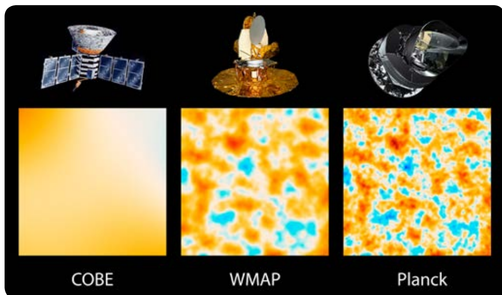
Anisotropy of Cosmic Microwave Background as seen by COBE, WMAP and Planck
