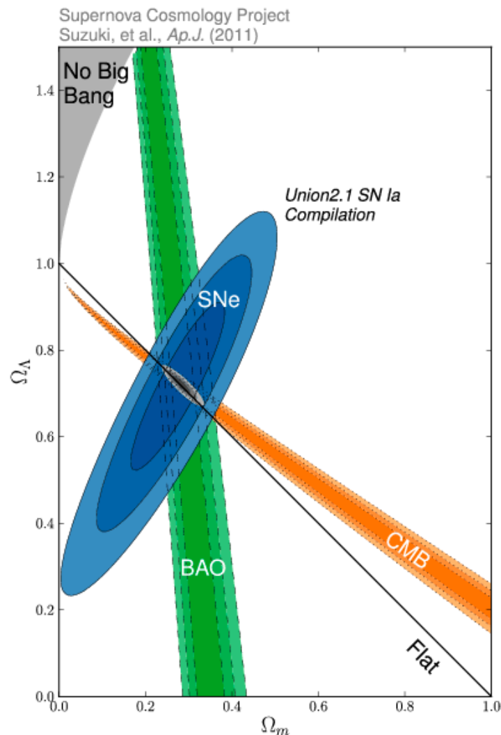
Allowed Dark Matter and Dark Energy bands in the Universe from various measurements.
