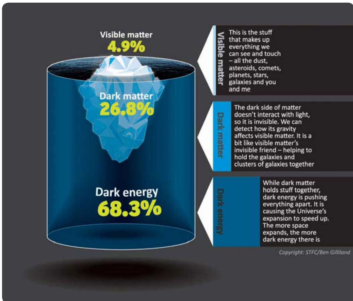
The relative abundances of the three presumed constituents of mass-energy in our Universe: visible matter, dark matter and dark energy (Credit: STFC/Ben Gilliland)
