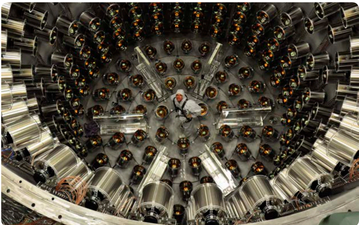
Core of the Double Chooz neutrino detector (Credit: CEA)
