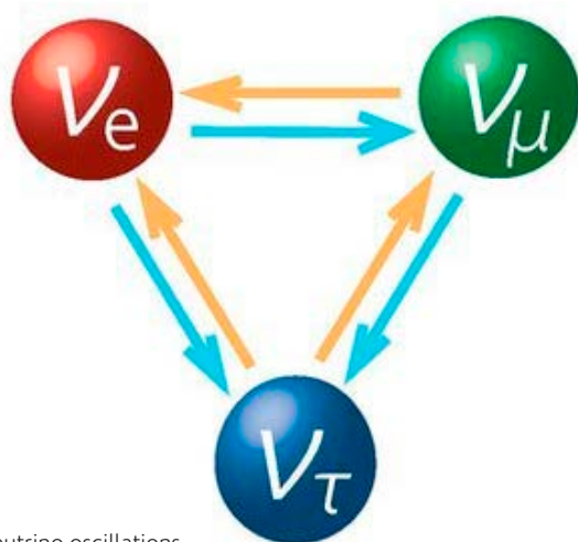
Neutrino oscillations
