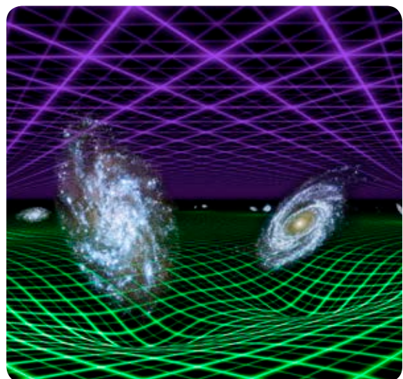
In this artist's conception, dark energy is represented by the purple grid above, and gravity by the green grid below. Gravity emanates from all matter in the universe, but its effects are localised and drop off quickly over large distances. Credit: NASA/JPL-Caltech
