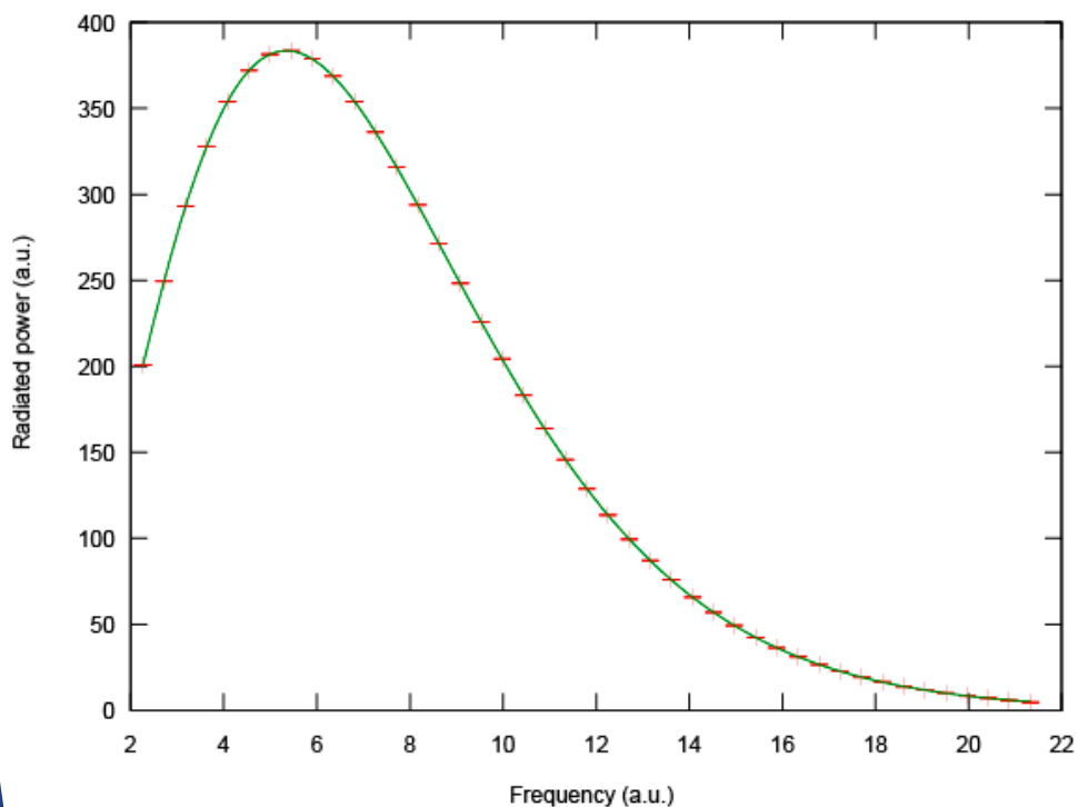
Radiated power as function of frequency of the cosmic microwave background as measured by the COBE satellite (points). The line shows the blackbody spectrum.
