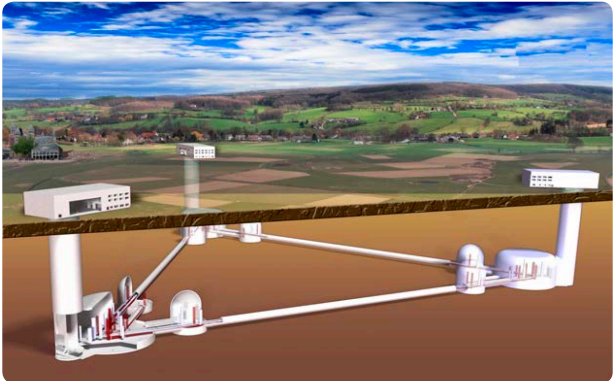
Artist's impression of the Einstein Telescope, a third-generation gravitational-wave (GW) detector (Credit: AEI)
